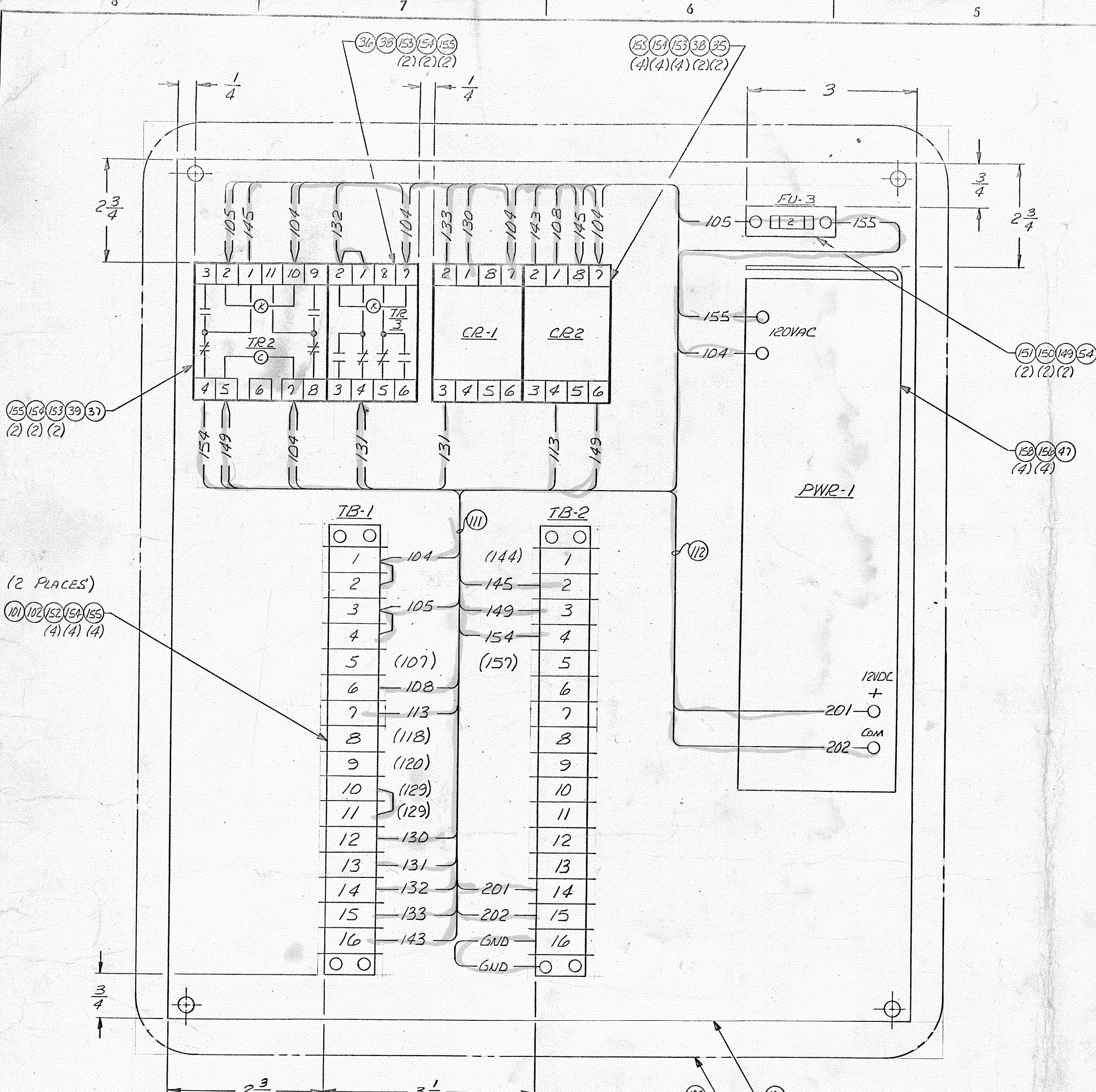
CONTROL SUPPORT EQUIPMENT PANEL ARR'GT & WIRING DIAGRAM
