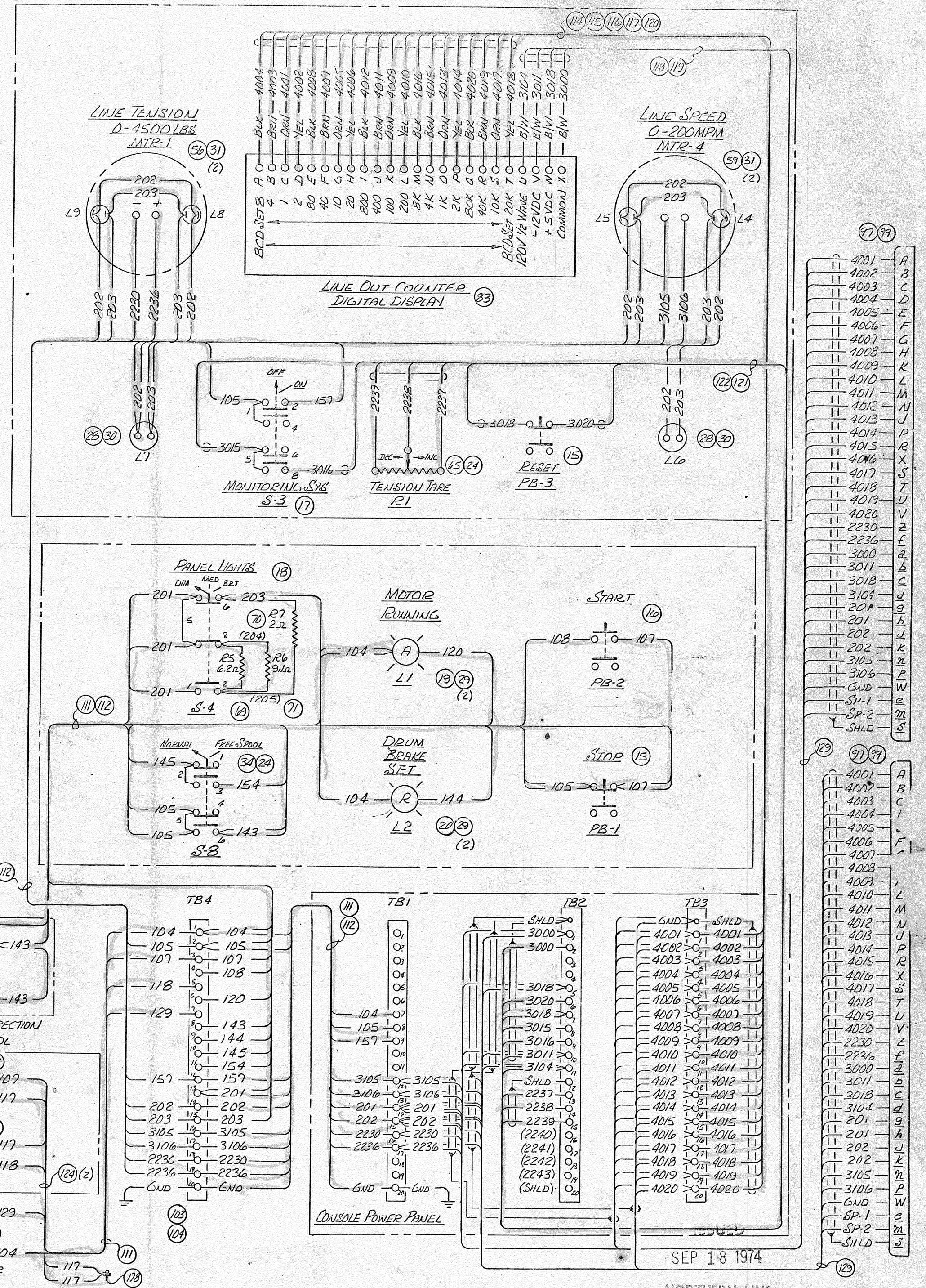
LOCAL CONSOLE, SUPPORT EQUIP PNL W/D & DETAILS HYDROWINCH, AGOR-22
